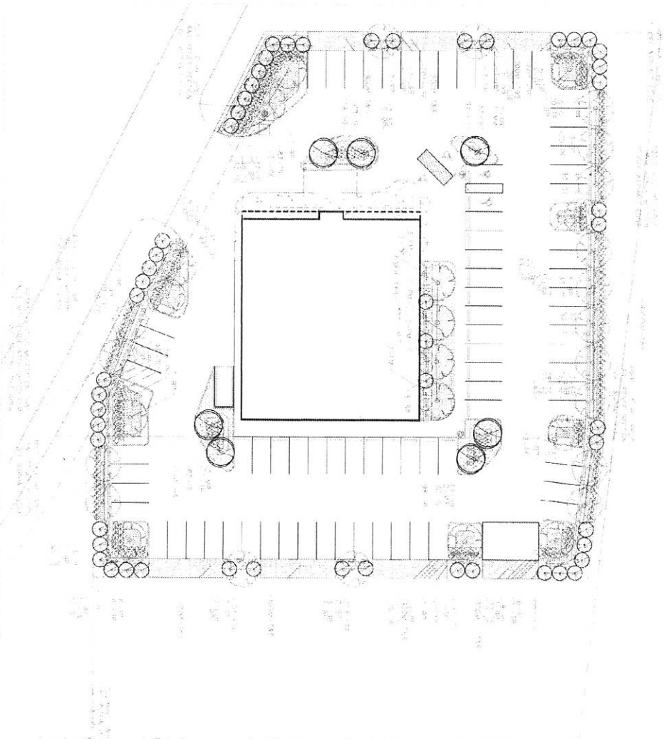
1 LANDSCAPE PLAN
