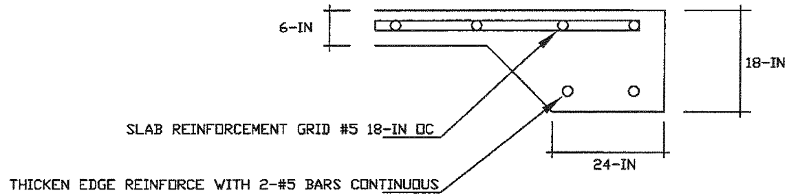
FOUNDATION END CROSS SECTION
